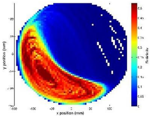
Figure 5: Transverse solidicity comparison. From Top: Pure DEM, One way coupled model, Two way coupled model Bottom: PEPT results.
