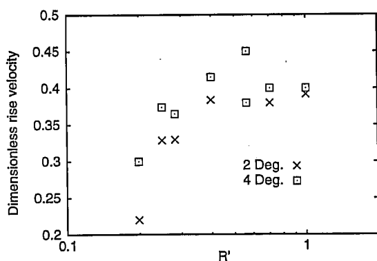
Figure 5: Non-dimensional bubble rise velocity (velocity divided by (g\mathcal{L})^{1/2} ) versus non-dimensional bubble size, R' .
