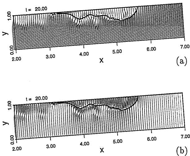
Figure 2: Instantaneous bubble shape and velocity vectors for bubble rise in a channel inclined at 4°: (a) Computational coordinate frame, (b) coordinate frame stationary with respect to the walls. Every fourth vector in each direction is displayed.
