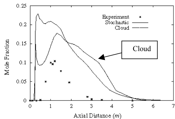
Figure 8: Comparison of CO mole fraction along the centerline of the reactor
