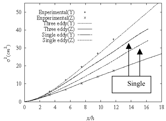
Figure 4: Comparison of single and three-eddy interaction model for fluid elements with experimental data of Huang and Stock (1997)
